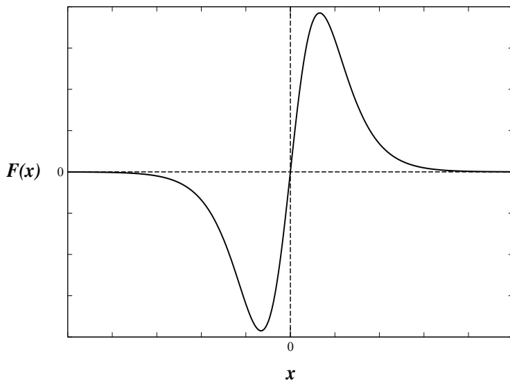
Figure 6: Perturbation F(x) given by Eq. (8) when 4B^2 > 1 .
