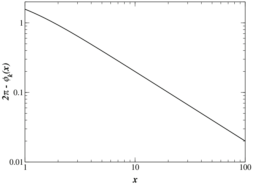
Figure 11: Asymptotic power law behavior of the kink solution. This is a log-log plot.
