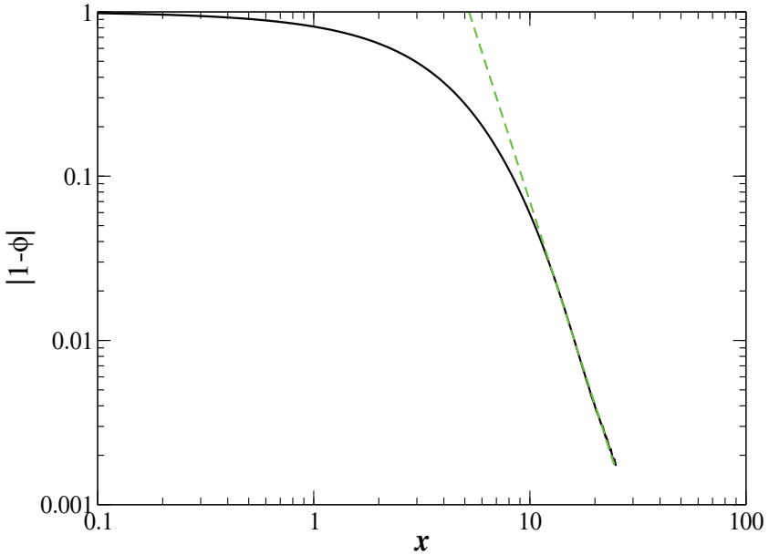
Figure 13: Log-log plot of the asymptotic behavior of the stabilized solution in the non-local Klein-Gordon equation with Q(x,y) = a[1 + b^2(x-y)^2]^{-1} .
