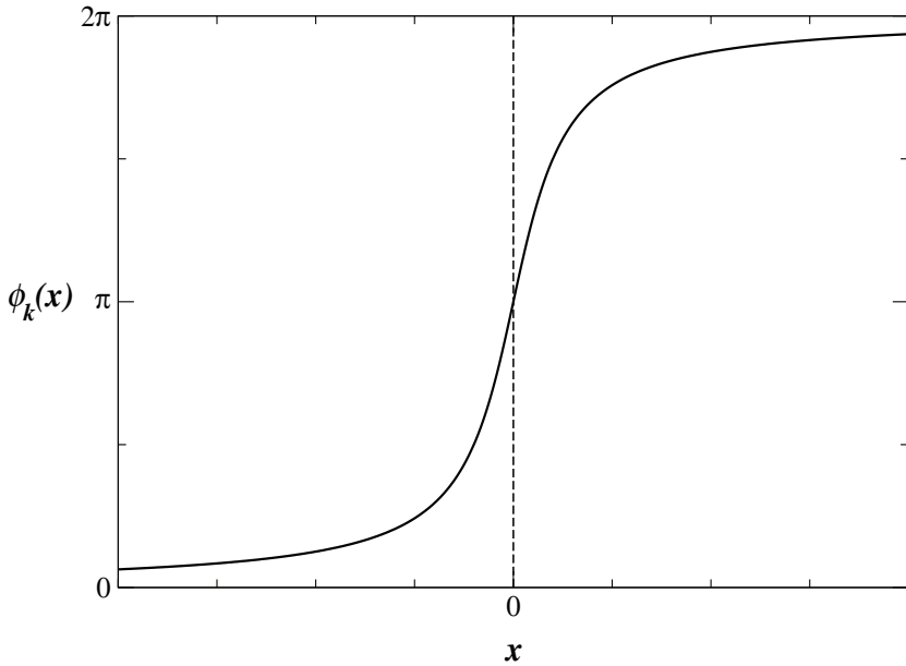
Figure 10: Kink solution for the potential U(\phi) = [(1 - \cos \phi)/2]^2/2 depicted in Fig. 9. The tail is a power law.
