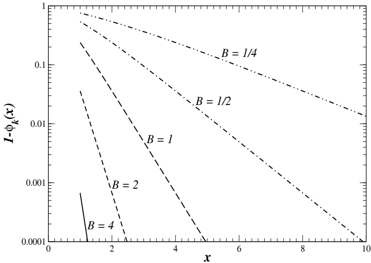
Figure 8: Asymptotic exponential behavior of the kink solution for different values of B . This is a simple log plot.
