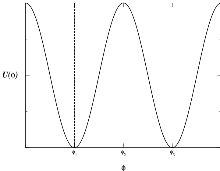
Figure 2: Potential U(\phi) for the generalized sine-Gordon equation.
