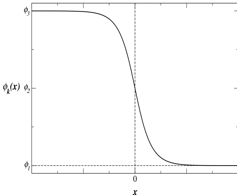
Figure 4: Antikink solution.
