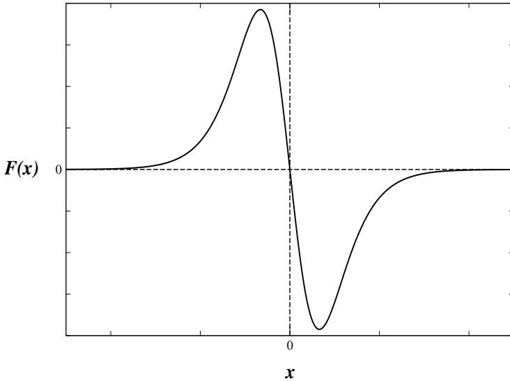
Figure 7: Perturbation F(x) given by Eq. (8) when 4B^2 < 1 .
