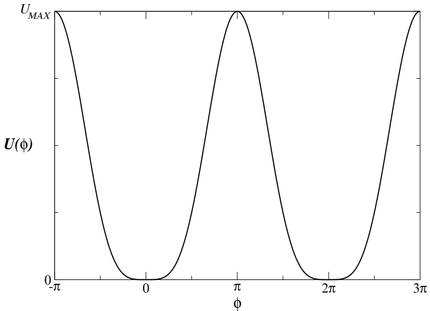
Figure 9: Potential U(\phi) = [(1 - \cos \phi)/2]^2/2 in Eq. (16). The kink-antikink interaction is long range for n > 1 .
