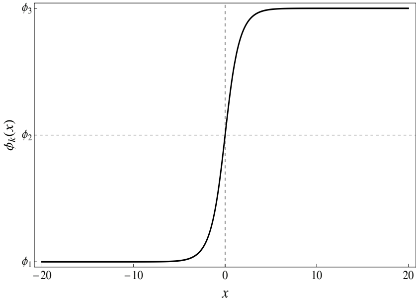
Figure 12: Kink-soliton solution for Klein-Gordon equation (23) with U(\phi) as in Eq. (24).
