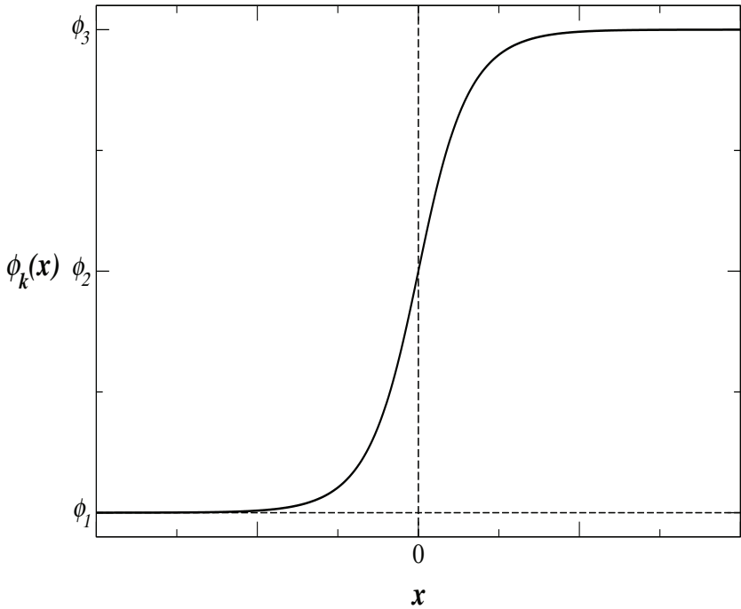
Figure 3: Kink solution.
