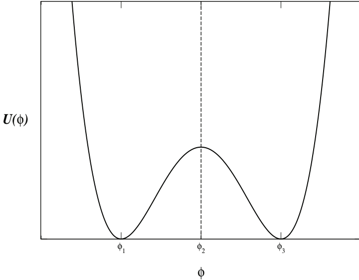
Figure 1: General potential U(\phi) in the generalized Klein-Gordon equation (1) for the existence of kink and antikink solutions.
