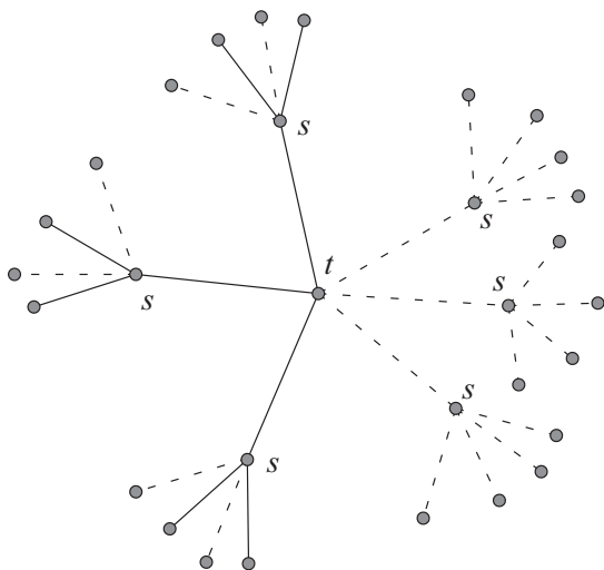
Figure 1: Example illustrating tree T_{t,s} for 2 \leq s < t < 2s .
