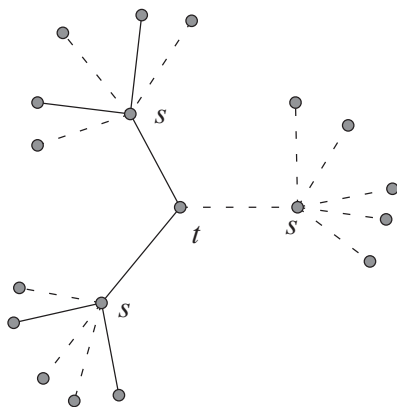
Figure 2: Example illustrating tree T_{t,s} for s > t \geq 2 .
