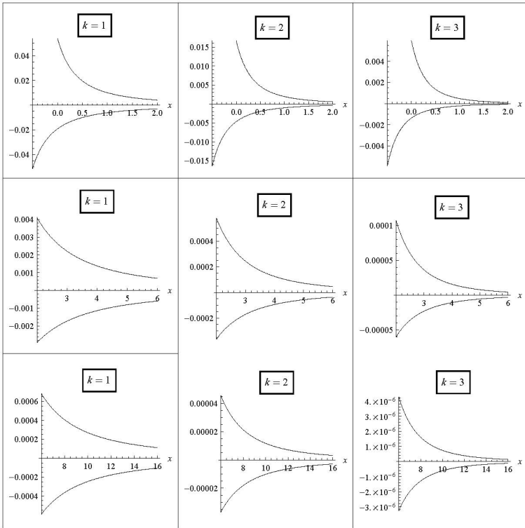
Figure 1. The relative errors of the bounds \mathcal{L}_k(x) and \mathcal{U}_k(x) for k \in \{1, 2, 3\} and x \in (-\frac{1}{2}, 16] .
