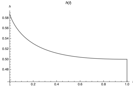
Figure 1: The graph of h(t) from (14) with p = 3/2 and r = 2 . Observe how this says that C_{3/2,2} = 1/2 .
