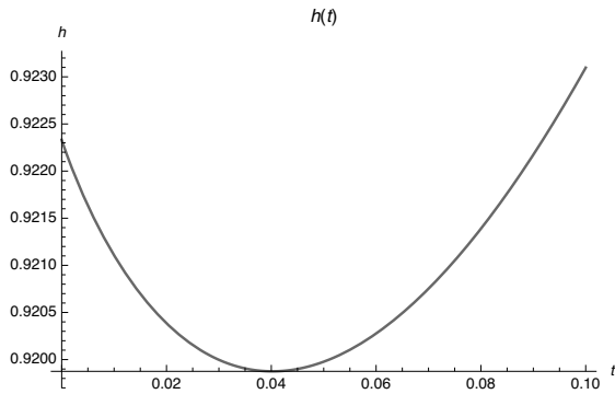
Figure 3: The graph of h(t) from (14) with p = 7/4 and r = 22/10 .
