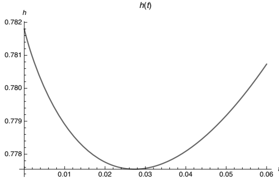
Figure 2: The graph of h(t) from (14) with p = 3/2 and r = 5/2 .
