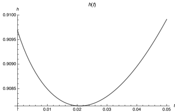
Figure 4: The graph of h(t) from (14) with p = 5/3 and r = 21/12 .
