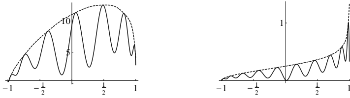
Figure 2: Graphs of \widehat{\Delta}_n(x)/(1-x) (solid line) and \Delta_n(x)/(1-x) (dashed) for n = 7 , \alpha = -\frac{3}{4} , \beta = -\frac{1}{4} (left) and n = 10 , \alpha = -\frac{1}{4} , \beta = 0 (right)
